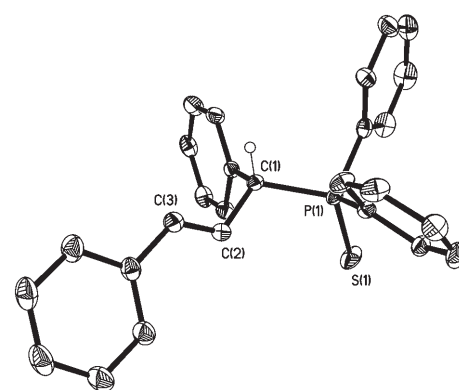
Figure 3. ORTEP diagram of the phosphine sulfide R - 20 . Hydrogen atoms are omitted for clarity, except for that at C(1); thermal ellipsoids are set at 30% probability.
