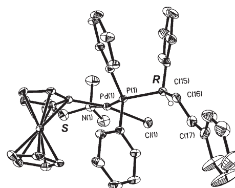
Figure 2. ORTEP diagram of compound 19 used for the determination of the absolute configuration of 4 . Only the hydrogen atom at the newly generated stereogenic center is shown at its calculated position; thermal ellipsoids set at 30% probability.
